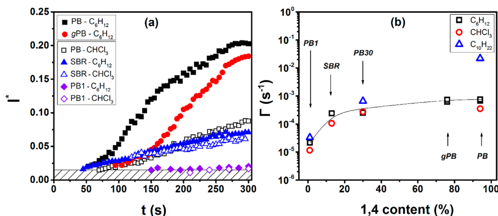
Figure 4. (a) Averaged normalized image intensity ( I^* ) as a function of laser illumination time for PB, gPB, SBR, and 1,2-PB solutions in C 6 H 12 and CHCl 3 . (b) Dependence of the growth rate \Gamma for formation of the structure on the 1,4 content of all of the used polymer solutions in C 6 H 12 , CHCl 3 , and C 10 H 22 .
