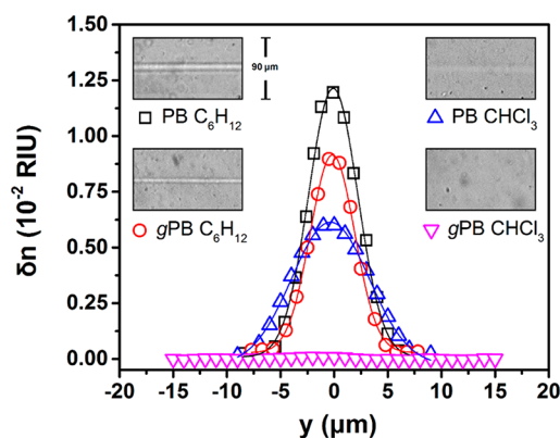
Figure 2. Phase contrast images (image size 169\ \mu\text{m} \times 90\ \mu\text{m} ) and corresponding refractive index profiles in PB and gPB solutions in \text{C}_6\text{H}_{12} (10 wt %) and in PB and gPB solutions in \text{CHCl}_3 (10 wt %) after 300 s of laser illumination.
